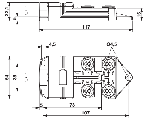
Dimensional drawing
